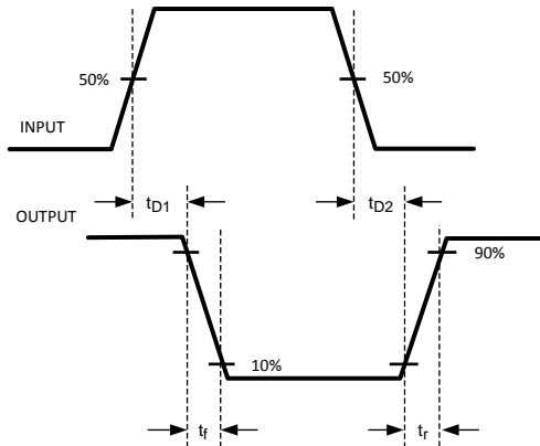
Figure 3. Inverting
